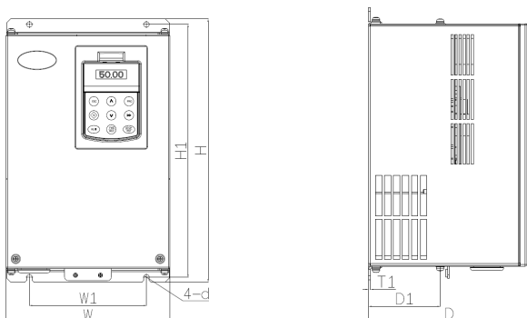
V6-H1-4T37G~V6-H1-4T 90G 功率等级
