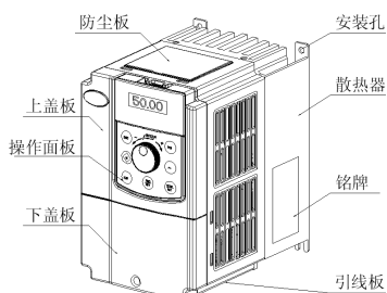
V6-H-2T0.4GX~V6-H-2T2.2GX V6-H-4T7.5GX/11LX 及以下功率等级
