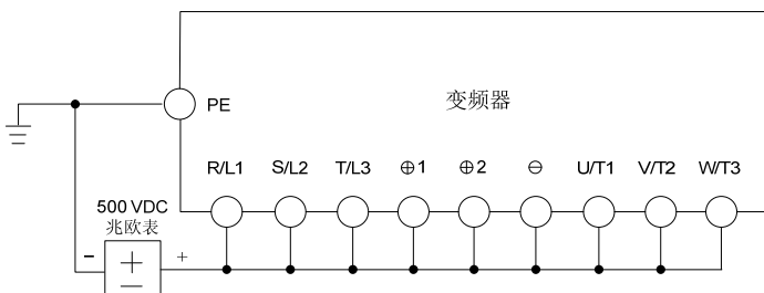
图8-2 V6-H-4T18.5 GX/22LX~V6-H-4T500GX/560LX主回路绝缘测试
