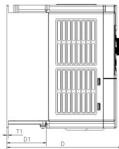
V6-H-2T0.4GX~V6-H-2T2.2GX、V6-H-4T7.5GX/11LX 及以下功率等级
